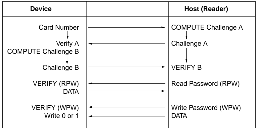
Figure 1. Security Methodology
