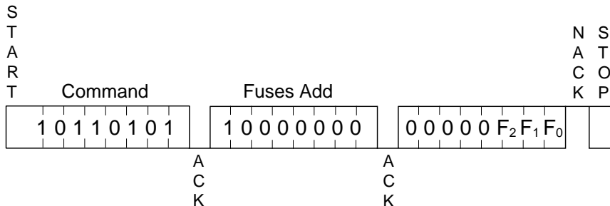
Figure 7. Read Fuses
